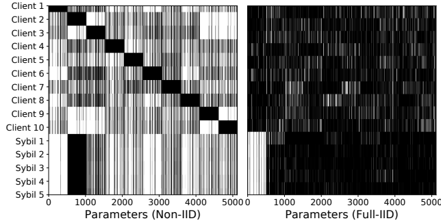
Figure 8: A visualization of the historical gradient of each clients on the Squeezenet model, in the non-IID (left) and IID (right) case. The top 10 rows show the gradient vector of honest clients; the bottom 5 rows for sybils performing a targeted 0-1 attack.
