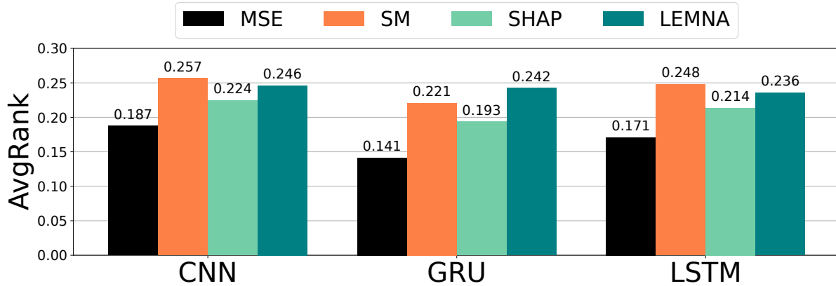
Figure 5.3: When attributing ICS anomalies at the time of detection, the raw-error feature (MSE) produces a lower AvgRank (lower is better) than all best-performing ML-based attribution methods: the saliency map (SM), SHAP, and LEMNA.
