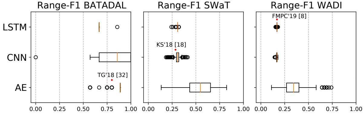
Figure 4.5: The final range-F1 scores of each model when trained and tuned on three experimental ICS datasets. For each dataset, a selected model hyperparameter setting from prior work is included for comparison.
