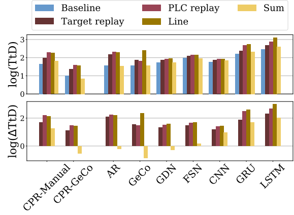
(d) Time-to-detect (lower is better) on TEP.
