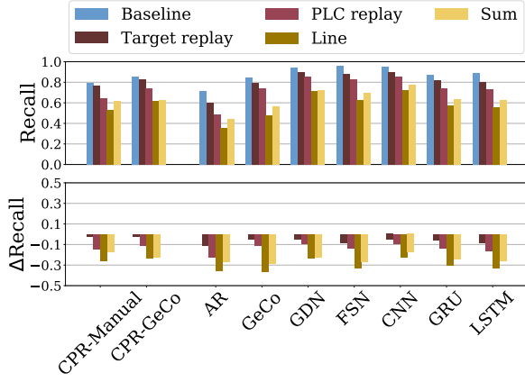
(c) Detection recall on TEP.
