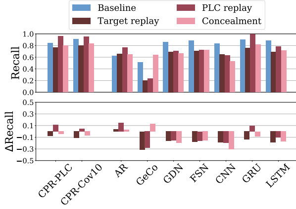
(a) Detection recall on CTown.
