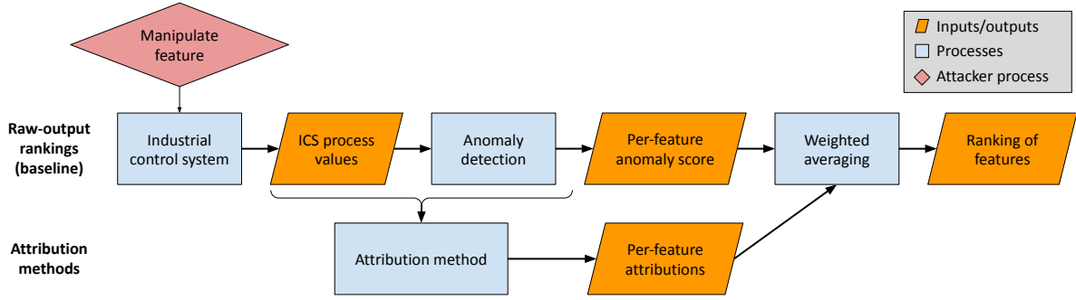
Figure 5.1: In this work, we describe and evaluate each step when attributing an ICS attack. Raw-output rankings (top) are the baseline method from prior work. We introduce ML-based attribution methods (bottom) as an alternative. We average and sort attribution scores to produce an overall ranking of suggested features for investigation.
