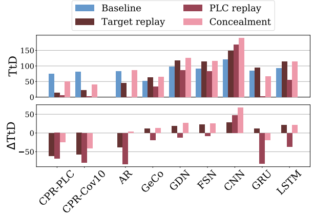
(b) Time-to-detect (lower is better) on CTown.
