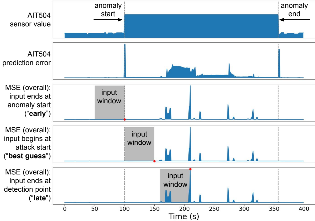
Figure 5.4: We show outputs of a GRU-based anomaly-detection model on SWaT attack #10: when sensor AIT504 is manipulated (top), its prediction error (2nd) is insufficient to trigger an anomaly. As the ICS responds and the total error increases, the model detects the anomaly over 100 seconds later. From this example, attributions can be computed at three points (shown in red) with corresponding input windows (shown in grey): at the anomaly start (3rd), when the input window coincides with the anomaly (4th), or when the anomaly is detected (5th, bottom).
