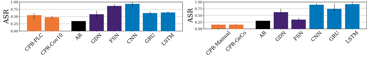
(a) Attack success rate for evasion attacks on the CTown dataset. (b) Attack success rate for evasion attacks on the TEP dataset.
