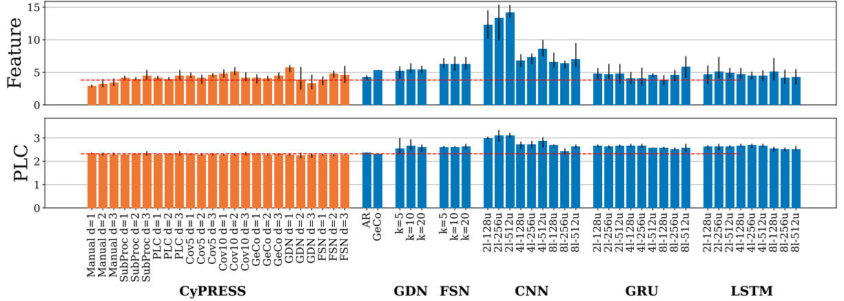
(b) Full attribution results on TEP.
