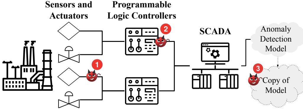
Figure 6.6: An overview of an ICS and the threat models we consider: attacks at the sensor level (#1), attacks at the PLC level (#2) and attacks that leverage knowledge of the anomaly-detection model (#3).
